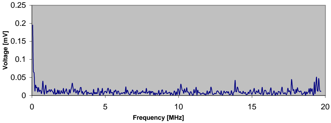
Frequency spectrum of the noise for channel 2 at 900V
