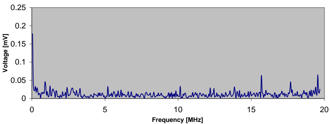
Frequency spectrum of the noise for channel 2 at 900V
