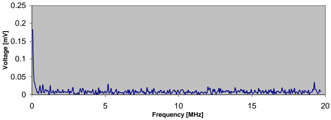
Frequency spectrum of the noise for channel 1 at 900V
