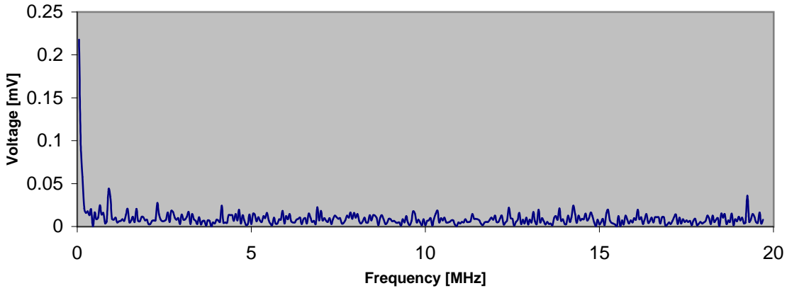
Frequency spectrum of the noise for channel 1 at 700V
