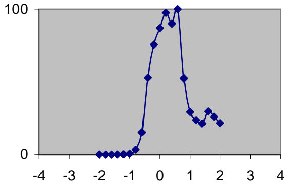
Noise distribution of HV power supply at 700V channel 2 after 15 hours of warming up
