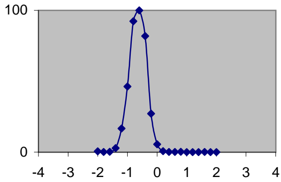
Noise distribution of HV power supply at 700V channel 1 after 15 hours of warming up
