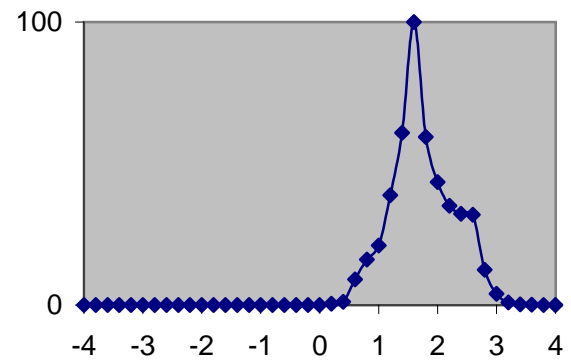
Noise distribution of HV power supply at 900V channel 2 after 15 hours of warming up
