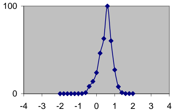
Noise distribution of HV power supply at 900V channel 1 after 15 hours of warming up
