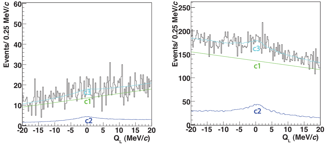
Figure 4: Background fit and signal extraction for \pi^- K^+ (right) and \pi^+ K^- (left) events.
