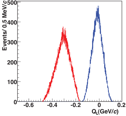
Figure 3: Q_L distribution of \pi^- K^+ events in blue and in red \pi^+ \pi^- events reconstructed as \pi^- K^+ events.
