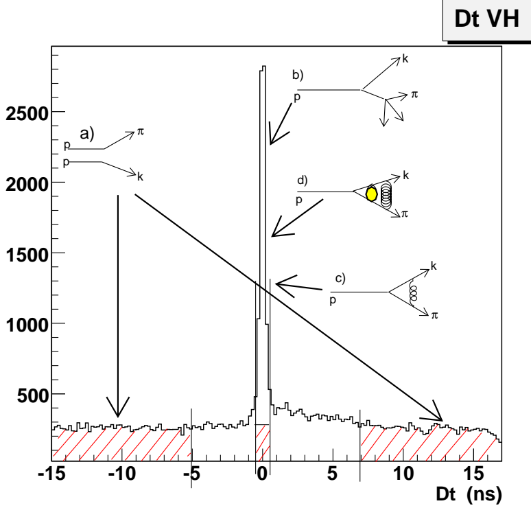
Figure 2: Time difference between the Vertical Hodoscopes for the \pi^\pm K^\mp final states.
