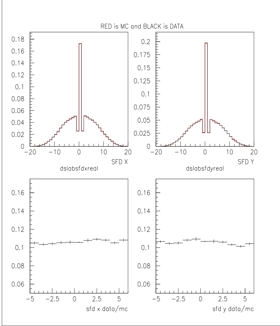
Figure 1: SFD simulation.
