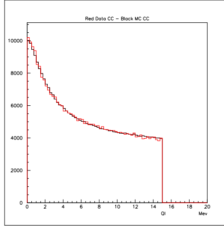
Figure 2: Q_l distributions for CC Data and Montecarlo.
