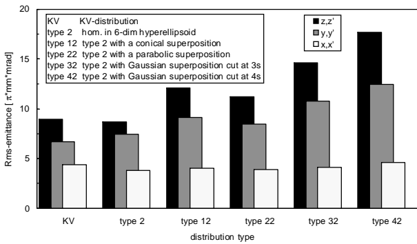
Fig. 8. Rms-emittance for different input particle distributions.
