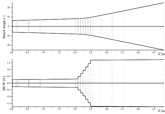
Fig. 3. Long. matching to the gas stripper, calculated for a KV-distribution with PARMT.
