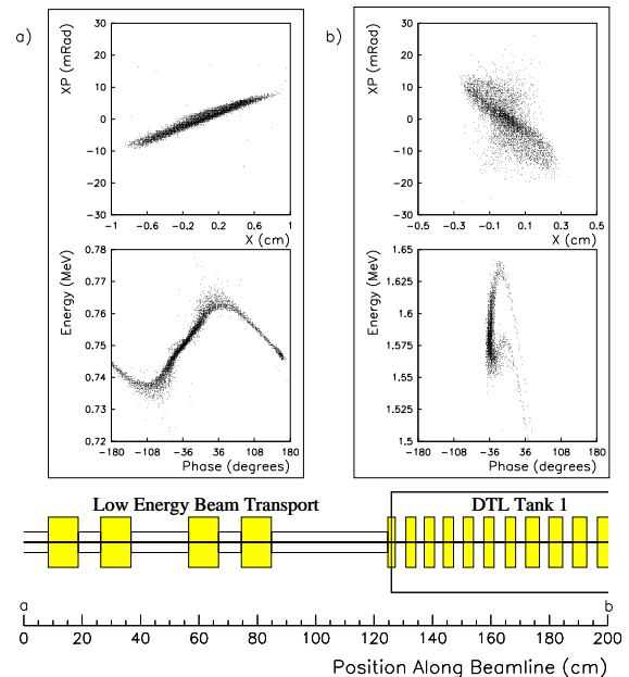
Fig. 1: (a) The horizontal and longitudinal phase-space distributions at the last emittance measuring station and (b) at the exit of the tenth drift tube for the standard quad and buncher settings. The bottom schematic diagram shows the end of the LEBT and the entrance to the DTL (shaded blocks are quadrupole magnets).
