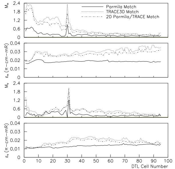
Fig. 3: Horizontal and vertical mismatch ( M ) and normalized emittance ( \epsilon ) versus drift tube number in the first two tanks of the DTL.
