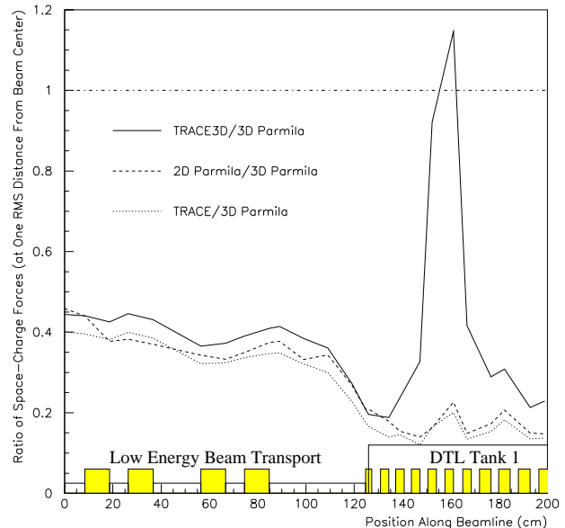
Fig. 2: The ratio of space-charge forces experienced by a particle at an RMS distance from the center of the bunch between TRACE, 2D PARMILA, TRACE 3-D and PARMILA.
