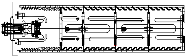
Figure 3. In an electrostatic quadrupole injector, the electrodes are arranged to accelerate and to focus the ion beams simultaneously.
