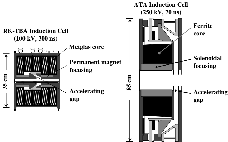
Figure 1. The RTA cell (100 kV, 300ns) is much more compact than the ATA cell (250 kV, 70 ns).
