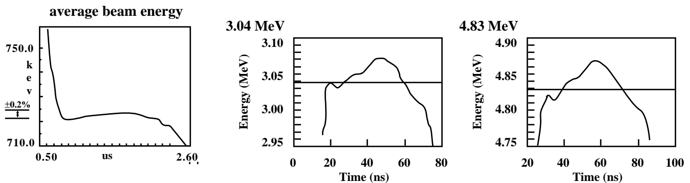
Figure 2. Energy spectrometer measurements for: (a) Ion beam from Heavy Ion Fusion Injector. (b) Electron beam from ITS at injector exit. (c) Electron beam from ITS after acceleration. Courtesy LANL for Figures 2(b) and 2(c).
