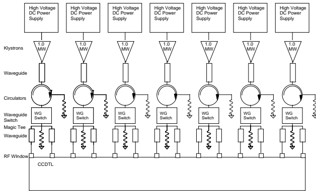
Fig. 3. Typical RF Super Module
