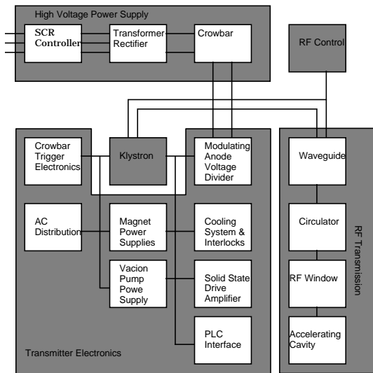
Fig. 2. RF system block diagram.
