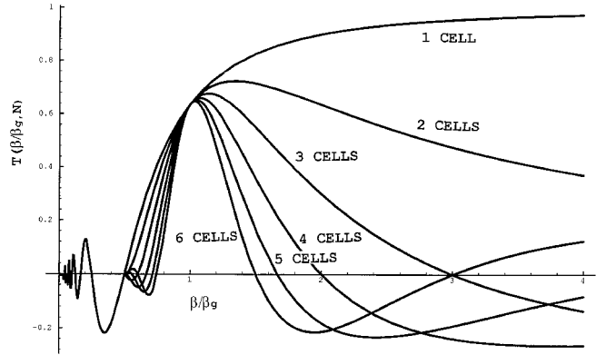
Fig. 1. Transit-time factor from the model versus \beta / \beta_G .
