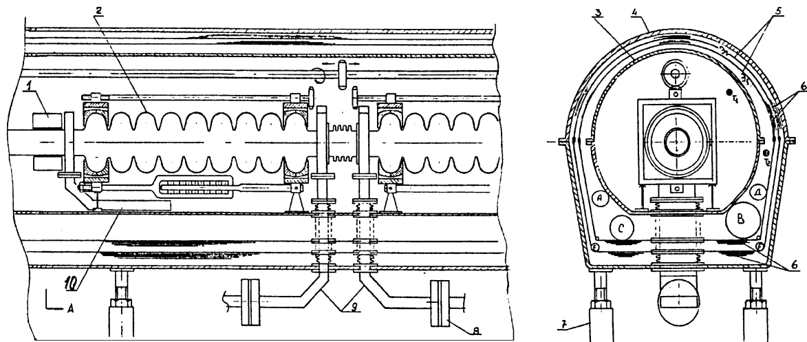
Fig. 1. 1 - quadrupole lens, 2 - accelerating cavity, 3 - helium vessel, 4 - cryo-module enclosure, 5 - heat ( \dot{Y}_2 ) and radiation ( \dot{Y}_1 ) screens enclosure, 6 - superisolation, 7 - supports, 8 - HF window, 9 - HF inputs system, 10 - load for high modes suppression, 11 - cavity adjusting mechanism, A, B, C, D, E, F - system of helium flow.
