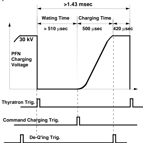
Fig. 3 Timing chart.
