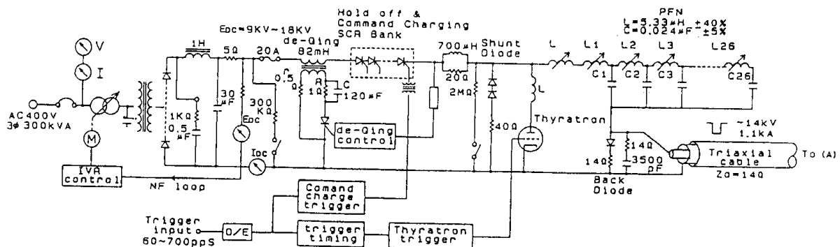
Fig. 1. Block diagram of the modulator.
