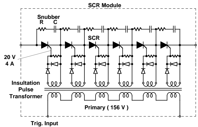
Fig. 4 Trigger circuit for SCR module.
