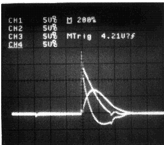
Fig. 6 Waveforms in de-Q'ing circuit. Channel 1 (top): de-Q'ing current on resistor, 300 A peak. Channel 2 (middle): total de-Q'ing current, 800 A peak. Channel 3(bottom): de-Q'ing current on capacitor, 800A peak. Ch. 1, Ch. 2, Ch. 3 = 200A/div, Time Base = 200 \mu s/div.
