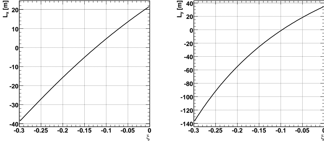
Figure 5: Effective lengths L_x(\xi) = \partial x(s)/\partial\Theta_x^* (left) and L_y(\xi) = \partial y(s)/\partial\Theta_y^* (right) at s = 145 m from IP5 as a function of the fractional proton momentum loss \xi .
