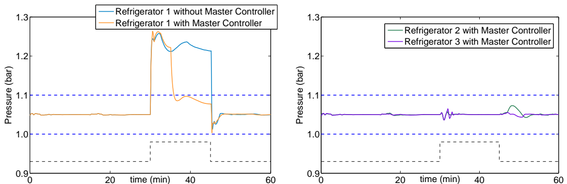
Fig. 4. Behavior of the low pressure when a sudden stop of one compressor (in refrigerator 1) takes place, with/without fault tolerance operation. The blue lines are the constraints, while the black dotted line symbolizes the time instant when the compressor is stopped.
