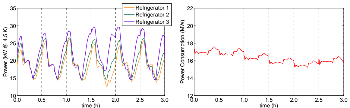
Fig. 3. Evolution of the refrigeration power provided by the three refrigerators and the total power consumption of the cryoplant, over 6 cycles; showing overall reduction in power consumption (around 7%), as desired. The dotted lines symbolize the ending of each cycle.
