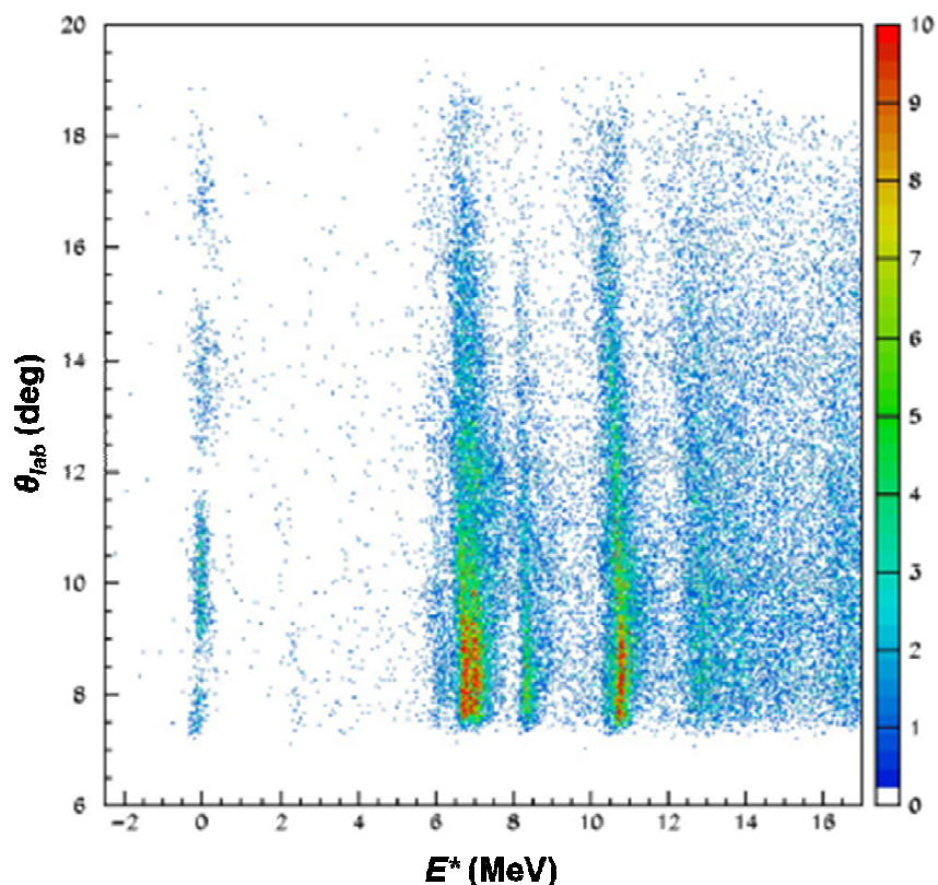
Figure 1. Two-dimensional plot of the reconstructed \theta_{lab} against the ^{14}\text{C} apparent excitation energy E^* for the ^{12}\text{C}(^{18}\text{O}, ^{16}\text{O})^{13}\text{C} reaction at 84 MeV.
