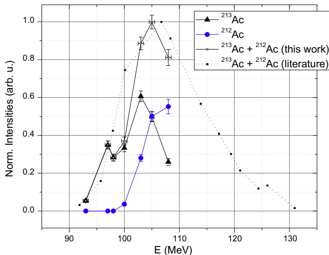
Fig. 6. Normalized production intensities of ^{212}\text{Ac} and ^{213}\text{Ac} as a function of the energy of the primary beam at the exit of the target. The summed function of the two isotopes is also shown for comparison with previous experimental results (see text).
