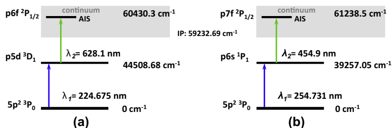
Fig. 2. Resonance ionization schemes for tin tested in these experiments. (a) Obtained by scanning the continuum in an atomic beam produced in the reference cell. (b) Taken from reference [21].
