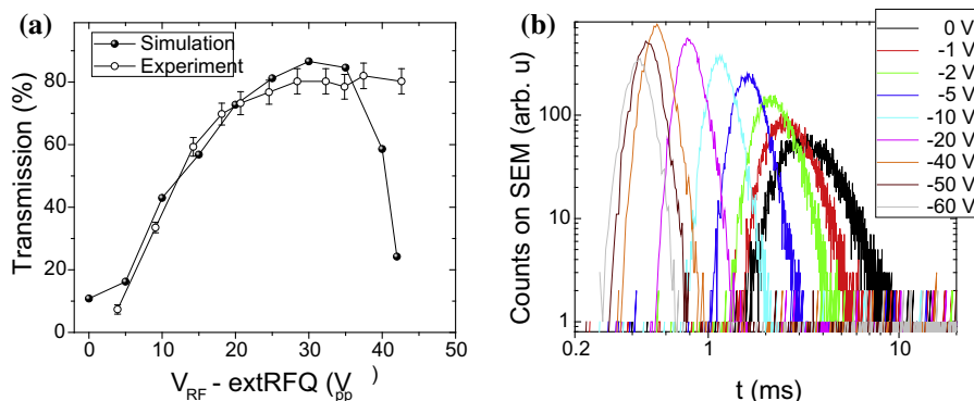
Fig. 8. (a) Simulated and experimental total transmission through the RFQ ion guides as a function of the RF amplitude applied to the extraction RFQ while operating the bent RFQ with an optimum value of the RF-amplitude of 300 V_{pp} . (b) Accumulated time profiles of a single laser shot registered on the SEM detector for different values of the DC potential applied between the first and last bent-RFQ segments.
