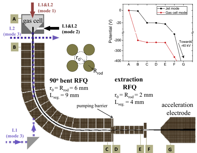
Fig. 7. Schematic layout of the prototype RFQ ion-guide system tested at LISOL. Ion trajectories through the system obtained with the SIMION ® software and the dimension of the RF electrodes are shown. The inset shows the evolution of the axial DC potential with reference to the different points indicated in the figure. Two alternative optical paths for laser ionization and spectroscopy are indicated (see text for details).
