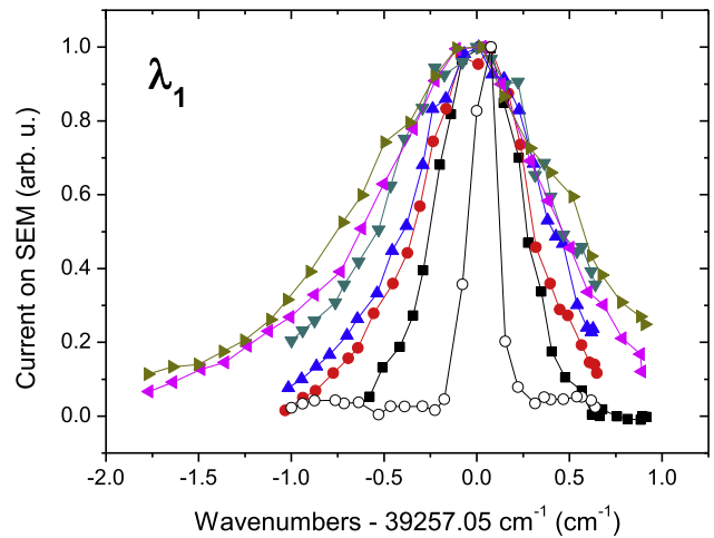
Fig. 3. Frequency dependence on the pressure for the first (bottom) and second (top) step transition in ^{120}\text{Sn} using the atomic scheme shown in Fig. 2b.
