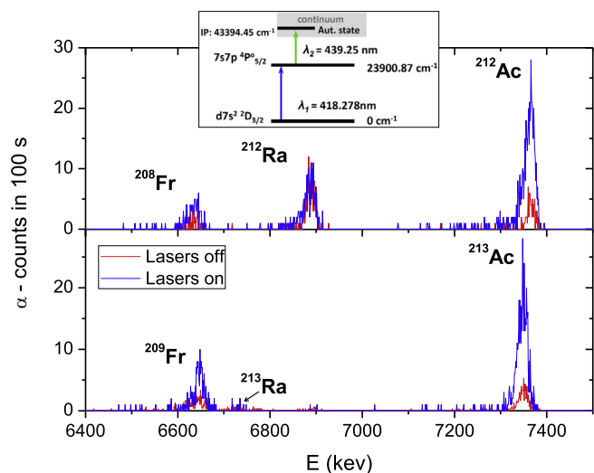
Fig. 5. Alpha spectra obtained when the mass separator was set to select ions with A/Q = 212 (top) and 213 (bottom). Characteristic lines for ^{212}\text{Ac} ( E = 7380 keV) and ^{213}\text{Ac} ( E = 7364 keV) may be seen for lasers on (blue) and lasers off (red). The main contaminant species along with the daughter decay products are also observed. The ionization scheme used in the production of the Ac beams is shown on top. (For interpretation of the references to colour in this figure legend, the reader is referred to the web version of this article.)
