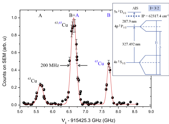
Fig. 9. Hyperfine splitting of the ^2P_{1/2} excited state for a natural mixture of copper isotopes produced in the reference cell. The relative peak intensities observed for ^{63}\text{Cu} and ^{65}\text{Cu} result from the naturally occurring isotopic abundance of 70% and 30%, respectively. The obtained linewidths were used to measure the reduction of the laser bandwidth by seeding of a CW diode laser into a pulse dye amplifier. The ionization scheme employed in these tests and the expected HFS of the electronic levels is shown in the inset.
