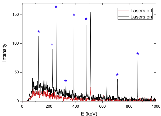
Fig. 4. Typical \gamma spectra obtained at the tape station when the mass separator was set to select a mass-to-charge ratio A/Q = 106 with lasers on resonance for the ionization of tin (dark) and with lasers off (light). The asterisks indicate characteristic \gamma peaks from the \beta decay of ^{106}\text{Sn} .
