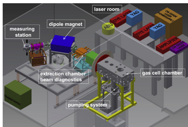
Fig. 10. Schematic layout showing the different components of the new laboratory that is being commissioned at KU Leuven for the study and optimization of the in-gas laser ionization and spectroscopy (IGLIS) technique to be used in on-line conditions at S 3 .
