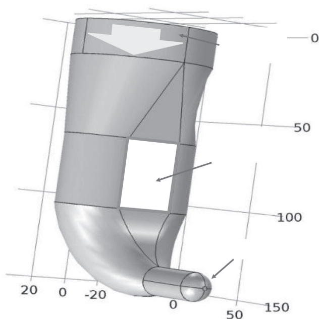
Fig. 11. Preliminary design of the new gas cell for S^3 . Dimensions are given in mm.
