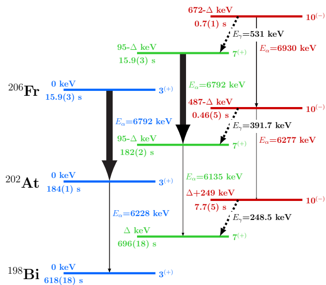
FIG. 2. \alpha -decay pattern of the ^{206}\text{Fr} - ^{202}\text{At} - ^{198}\text{Bi} decay chain [18]. Only the transitions relevant to the \alpha -decay tagging of the hyperfine components are presented. The dashed arrows represent \gamma decay and the full arrows \alpha decay, whereby the width is proportional to the branching ratio. Note the spins of ^{202g}\text{At} and ^{198g}\text{Bi} are the newly assigned 3^{(+)} , instead of (2,3^+) .
