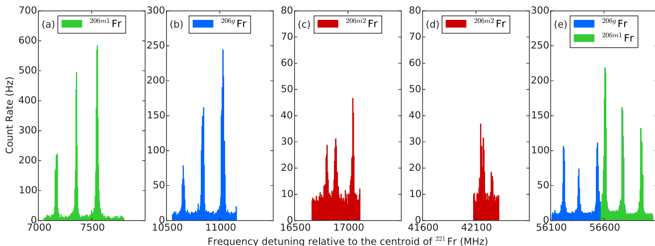
FIG. 1. Collinear resonance ionization spectroscopy of the low lying states of ^{206}\text{Fr} , relative to the centroid frequency of ^{221}\text{Fr} . The spin 3^{(+)} state is shown in blue [(b) and (e)], the spin 7^{(+)} state is shown in green [(a) and (e)], and the spin 10^{(-)} state is in red [(c) and (d)].
