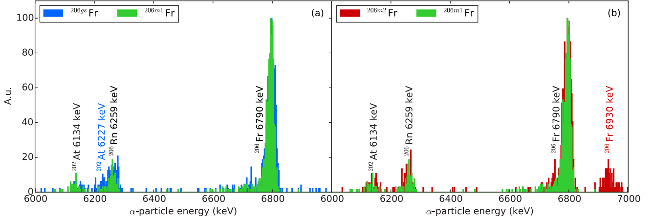
FIG. 3. \alpha -decay energy spectra of laser-separated beams of ^{206}\text{Fr} and its isomers, normalised to the 6790 keV peak. (a) Hyperfine components of laser-separated ^{206g}\text{Fr} and ^{206m1}\text{Fr} . The excess in \alpha particles at 6135 keV (6228 keV, respectively), is characteristic of the decay of the (7^+) [ (2,3^+) , respectively] state in ^{202}\text{At} , arising from the decay of the 7^{(+)} ( 3^{(+)} , respectively) state in ^{206}\text{Fr} . (b) Hyperfine components of ^{206m1}\text{Fr} and ^{206m2}\text{Fr} . The excess in \alpha particles at 6930 keV is characteristic of the decay of the 10^{(-)} state in ^{206}\text{Fr} .
