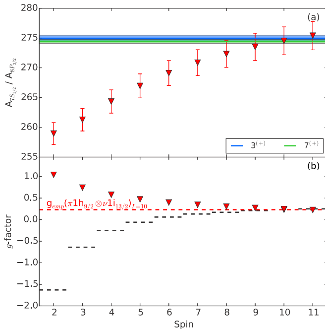
FIG. 4. (a) Ratio of the hyperfine A factors for the 7s^2S_{1/2} and 8p^2P_{3/2} electronic states of ^{206m2}\text{Fr} , for different nuclear spins ( I = 2^- to 11^- ). The blue line represents the ratio for ^{206g}\text{Fr} and the green line for ^{206m1}\text{Fr} . (b) The expected g factors for the different nuclear spins for ^{206m2}\text{Fr} , alongside the established g factors for the ( 10^- ) state in ^{202,204}\text{Fr} . The dashed lines give the empirically calculated g factor for each spin. See text for details.
