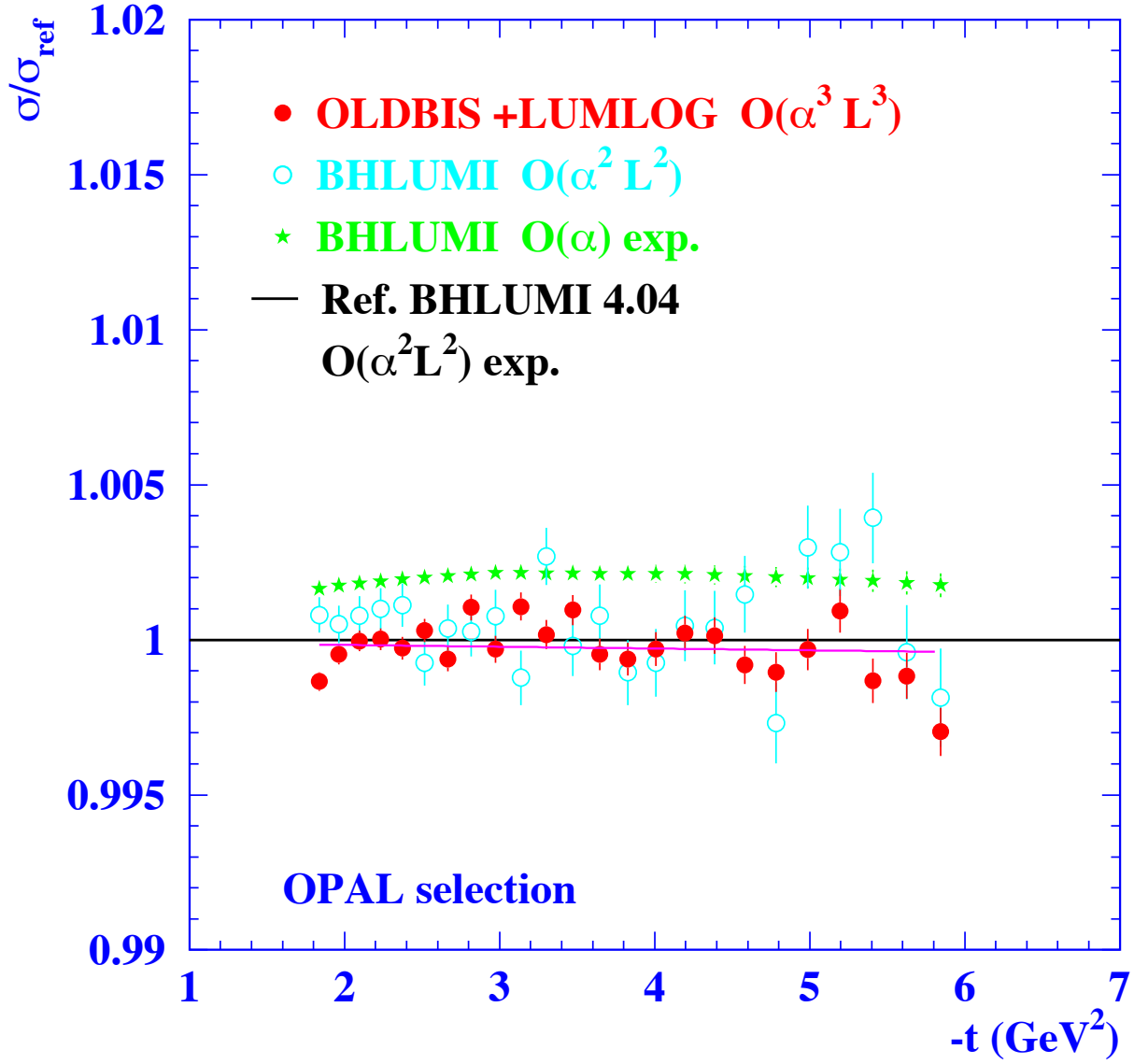
Figure 11: Differential cross section as a function of -t calculated by the BHLUMI package for the OPAL selection in different perturbative approximations, normalized to the reference BHLUMI calculation. Vacuum polarization, Z-interference and s -channel photon exchange contributions are switched off. The superimposed line is a fit to the OLDBIS+LUMLOG result.
