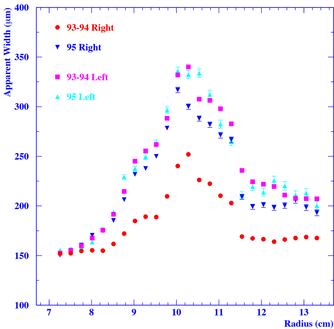
Figure 5: The apparent width \sigma_a as a function of radius determined from the anchoring procedure for the Si Layer at 4 X_0 for homogeneous data sets. The errors are statistical only.
