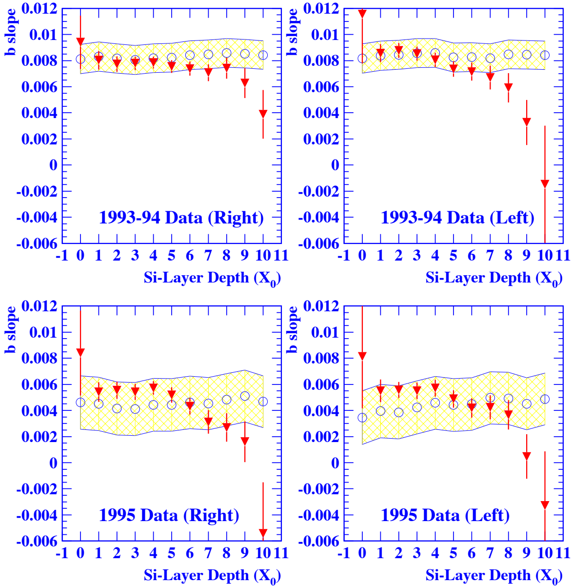
Figure 9: Fitted values of b as a function of the anchoring layer for homogeneous data combinations. The open circles show results obtained from uncorrected radial distributions, with the hatched band representing the (correlated) statistical error. The solid triangles show results from distributions corrected by anchoring, with the error bars representing only the systematic errors.
