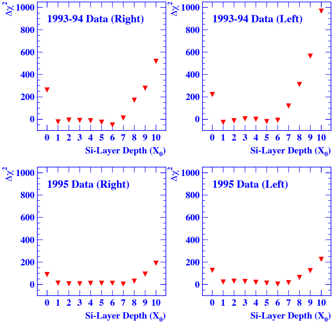
Figure 8: Difference between the corrected and uncorrected \chi^2 (d.o.f.=22) as a function of the anchoring layer for homogeneous data subsamples. Only statistical errors are considered.
