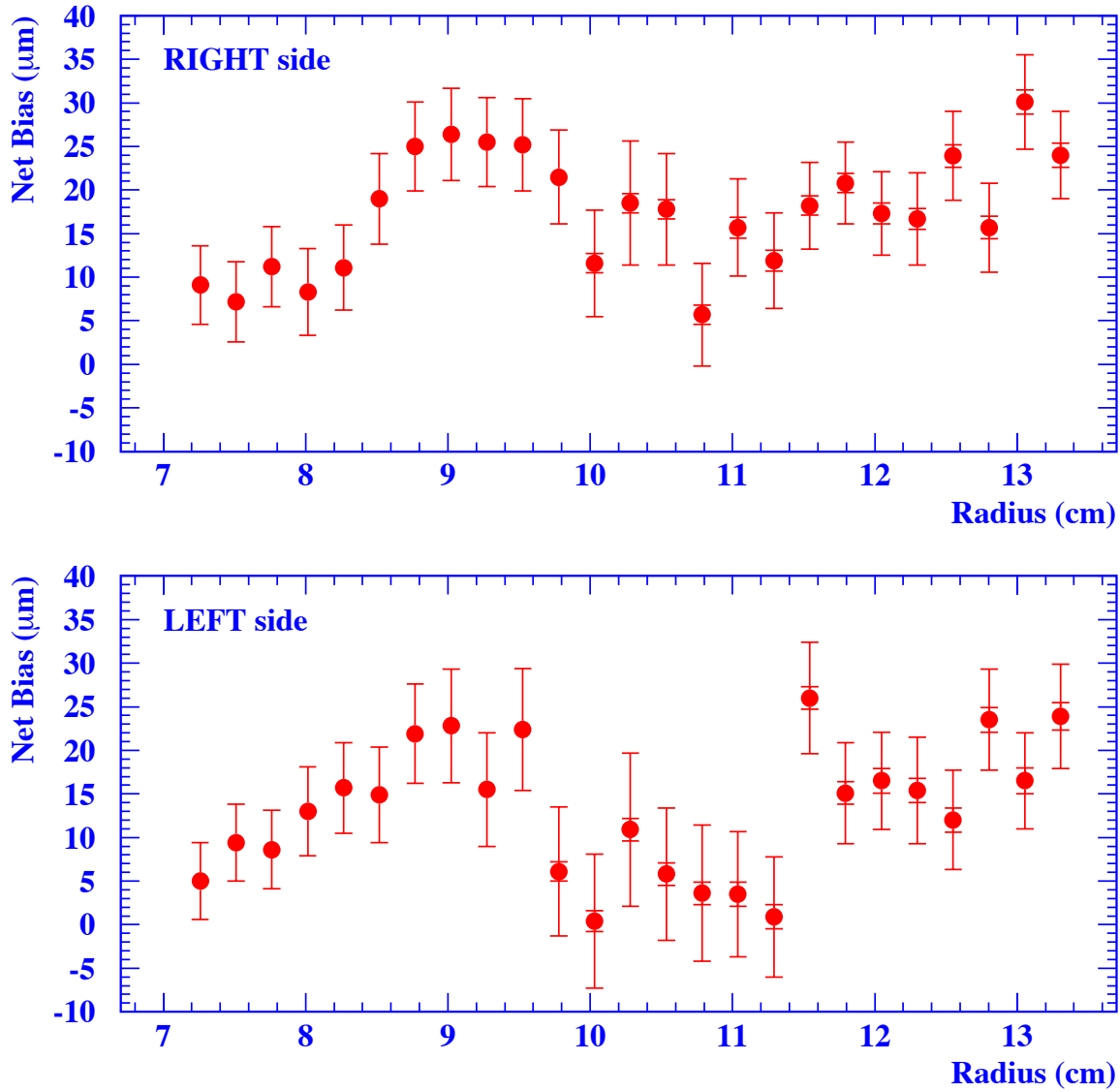
Figure 4: The total net bias ( anchor ) as a function of radius for the Right and the Left radial coordinate determined for the pad boundaries in the Si layer at 4X_0 , for the combined 1993-94 data sample. The full error bars show the total error, the inner bars the statistical component.
