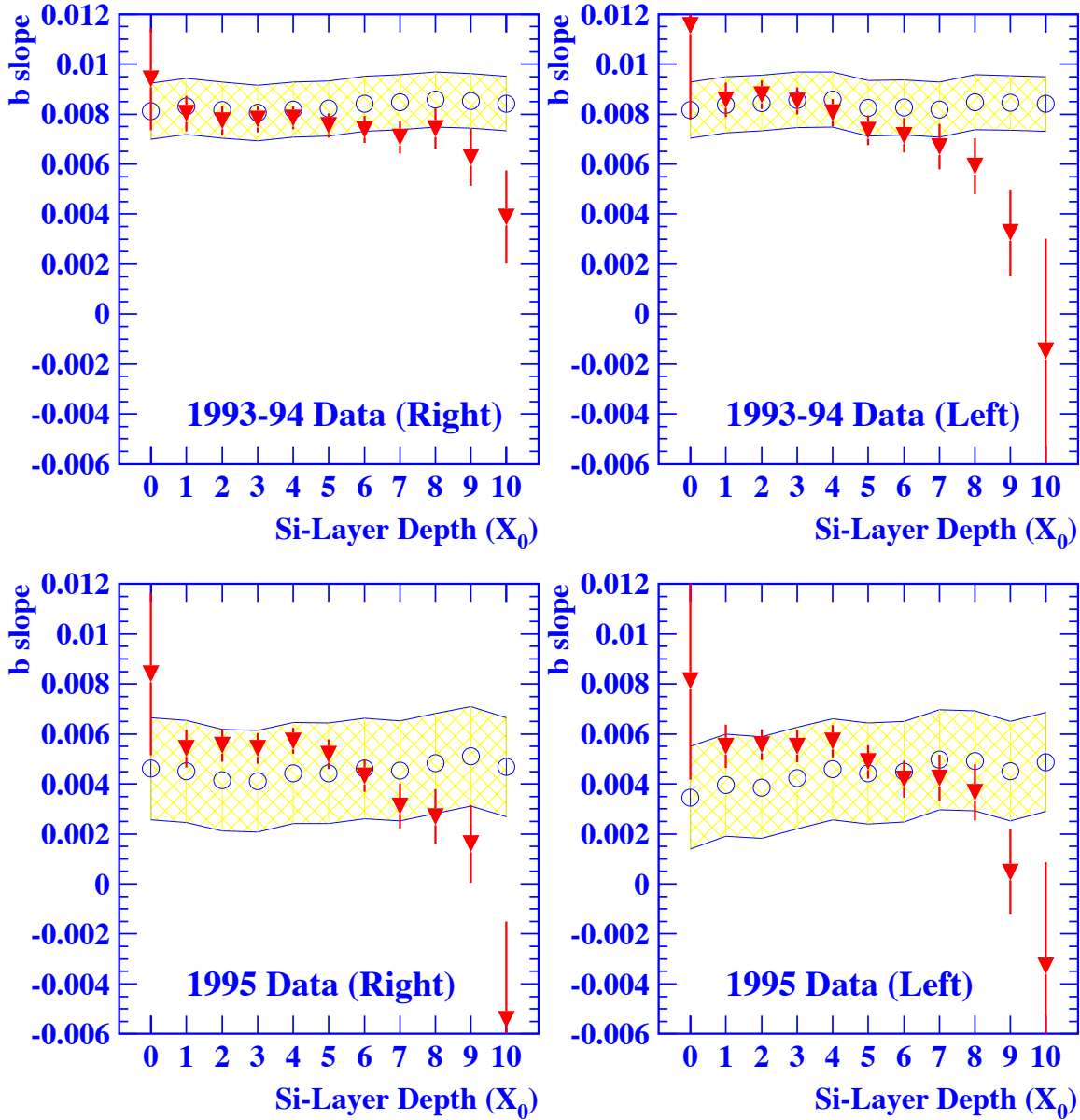
Figure 9: Fitted values of b as a function of the anchoring layer for homogeneous data subsamples. The open circles show results obtained from uncorrected radial distributions, with the hatched band representing the (correlated) statistical error. The solid triangles show results from distributions corrected by anchoring, with the error bars representing only the systematic errors.
