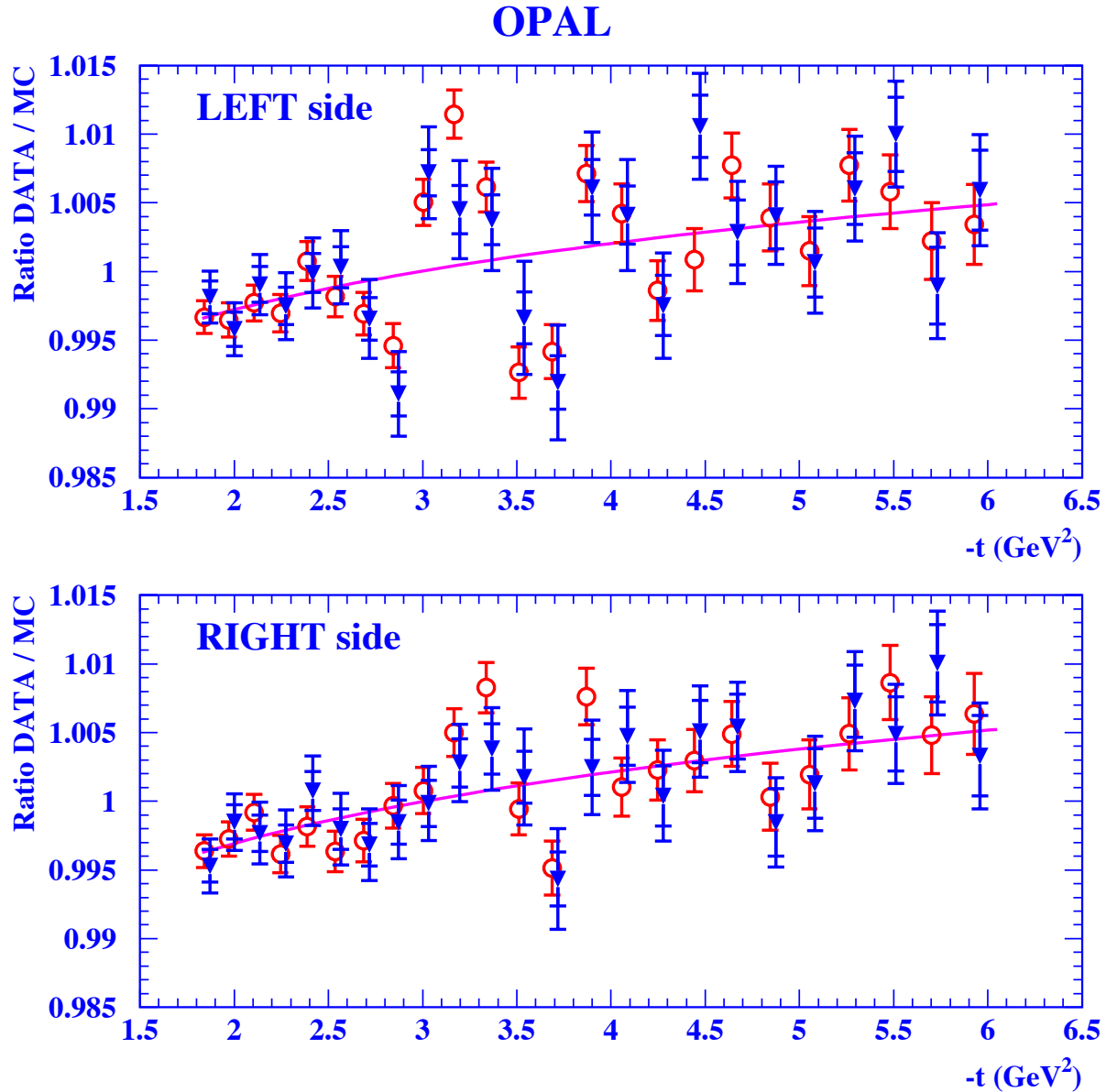
Figure 8: Ratios of numbers of data and Monte Carlo events (with \Delta\alpha set to zero) for the combined 1993-94 data sample, for the Left and Right sides. Each point corresponds to a bin of one radial pad. The solid triangles show the data corrected with anchors in layer 4 X_0 with total errors (the inner bars show the statistical errors), the empty circles the unanchored data (slightly shifted horizontally for clarity), with statistical errors. The line shows the fit to the anchored data.
