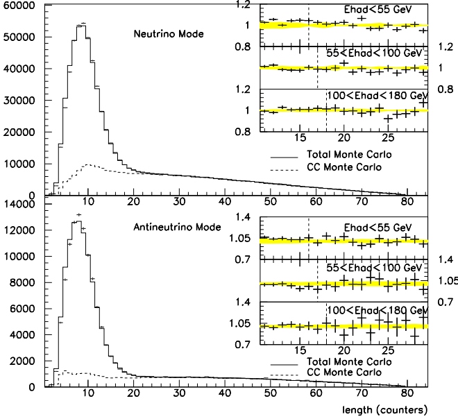
FIG. 1. Comparison of \nu and \bar{\nu} event length distributions in data and Monte Carlo (MC). The MC prediction for CC events is shown separately. Insets show data/MC ratio comparisons in the region of the length cut with bands to indicate the 1\sigma systematic uncertainty in this ratio.
