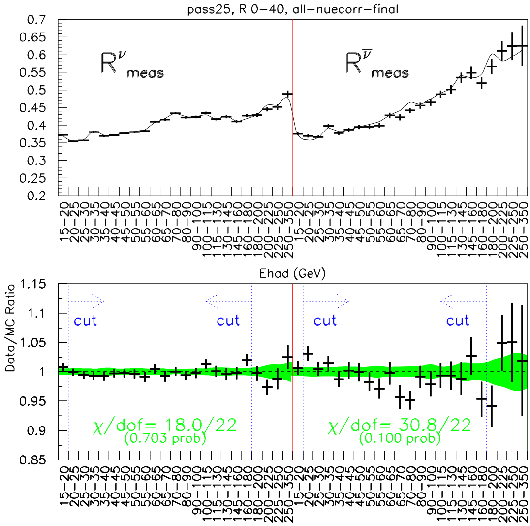
Figure 5: The R_{exp} as a function of visible energy in the neutrino and anti-neutrino beams. The ratio of data to Monte Carlo is shown below, with a green band to represent the systematic uncertainties in the comparison.
