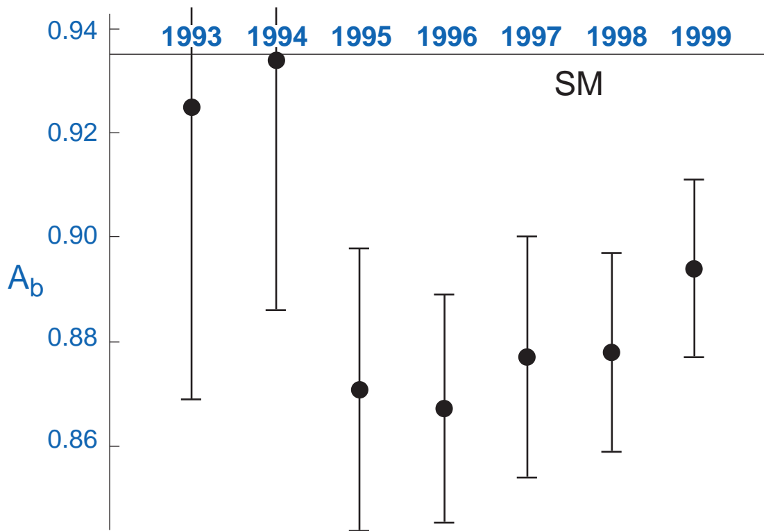
Figure 1: The time evolution of the LEP+SLD average value of A_b . The horizontal line shows the Standard Model prediction A_b = 0.935 .
