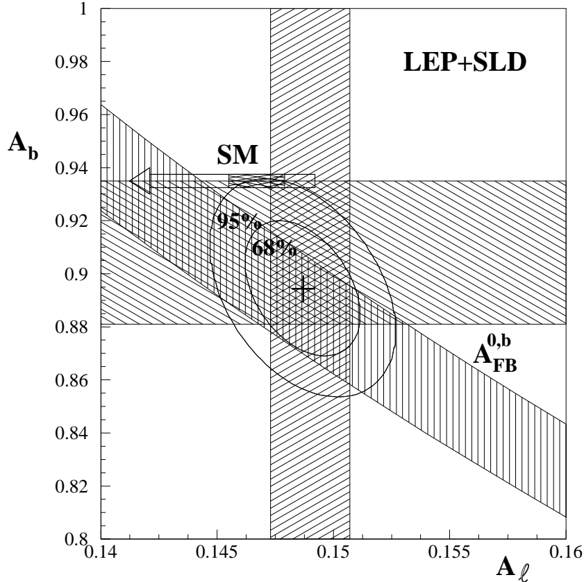
Figure 7: A_b versus A_\ell plot for LEP+SLD data. The cross shows the best fit value A_\ell = 0.1487 , A_b = 0.894 . WA and the SM arrow are defined as in Fig 5. The 68% and 95% CL contours of the fit are shown.
