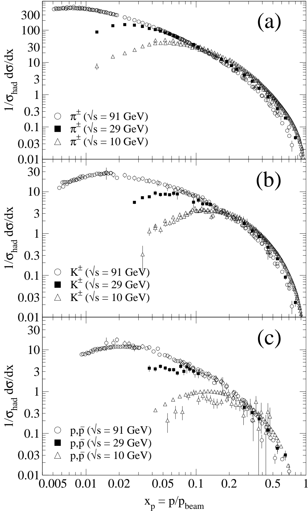
Figure 19.8: Scaled momentum spectra of (a) \pi^\pm , (b) K^\pm , and (c) p, \bar{p} at \sqrt{s} = 10, 29, \text{ and } 91 GeV [24, 26, 85, 161, 162].
