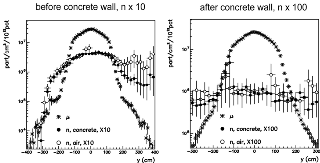
Figure 5.2 - FLUKA simulation results of particles in the first muon detector chamber. Muons and neutrons are compared before and after a concrete separation wall
