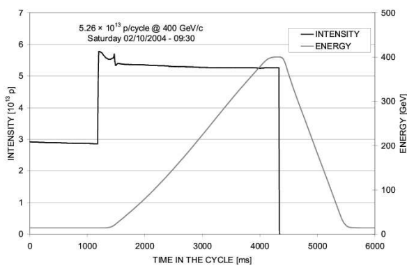
Figure 2: Beam transmission in the SPS at the end of the run. Transition crossing at \gamma_t = 22.8 , t=1485 ms.
