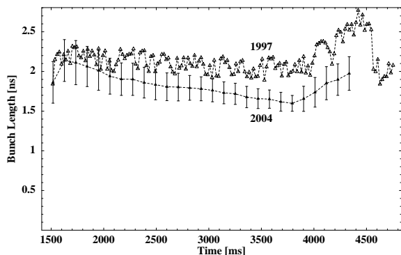
Figure 1: Bunch length evolution during the ramp starting from transition before (top trace) [6] and after (bottom trace, average for one batch) impedance reduction in the SPS . Voltage is around 7 MV in both cases. The total intensity is 4.1 \times 10^{13} and 5.1 \times 10^{13} correspondingly. Extraction at 400 GeV/c in 2004 and 450 GeV/c in 1997.
