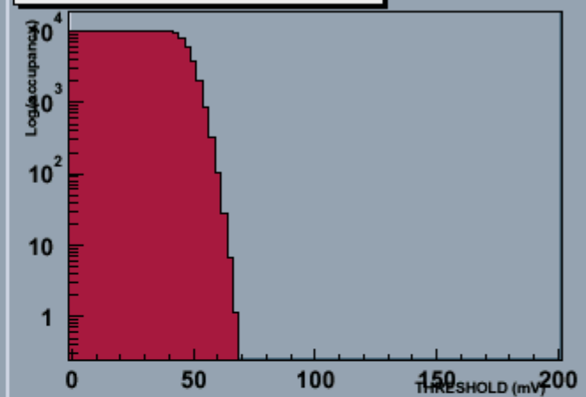
Module 1 80050000000763hDaqPR Stream 1 THRESHOLD (mV) Scan
