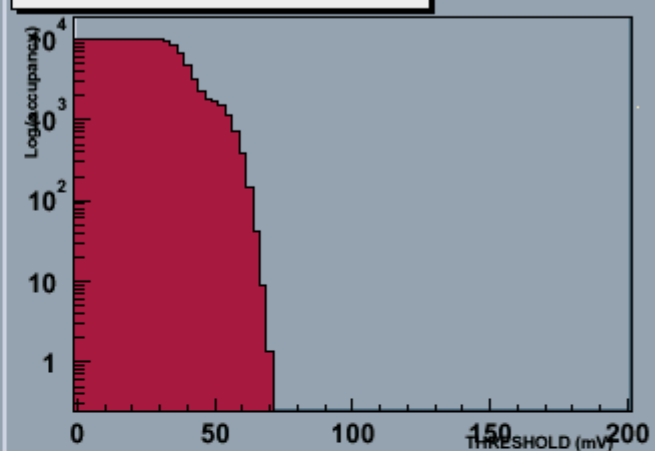
Module 3 6000000000754hDaqPRL Stream 1 THRESHOLD (mV) Scan
