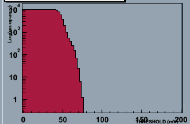
Module 1 80050000000763hDaqPR Stream 1 THRESHOLD (mV) Scan
