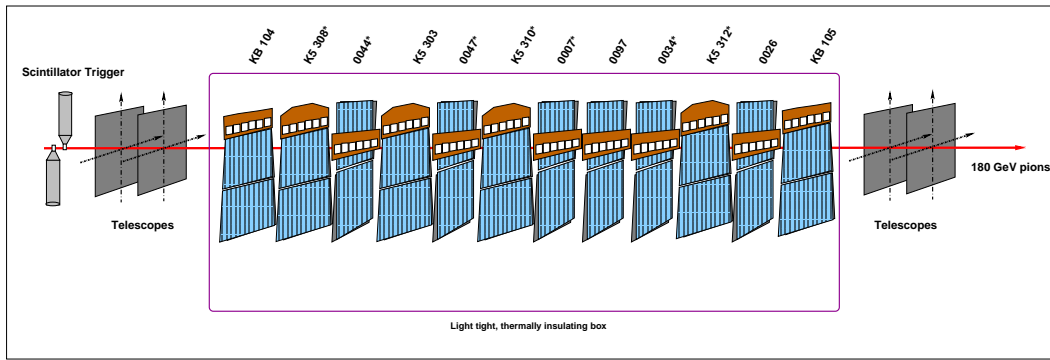
Fig. 1. Arrangement of the SCT prototype modules in the beam line during the tracking study.
