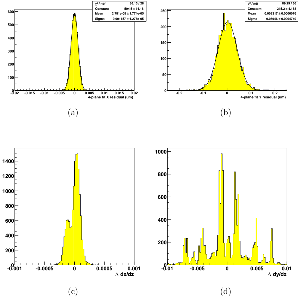
Fig. 4. Difference in track parameters between the track reconstructed from the beam telescope information and from a four-barrel-module array: (a) X position (b) Y position (c) X slope wrt beam axis (d) Y slope wrt beam axis
