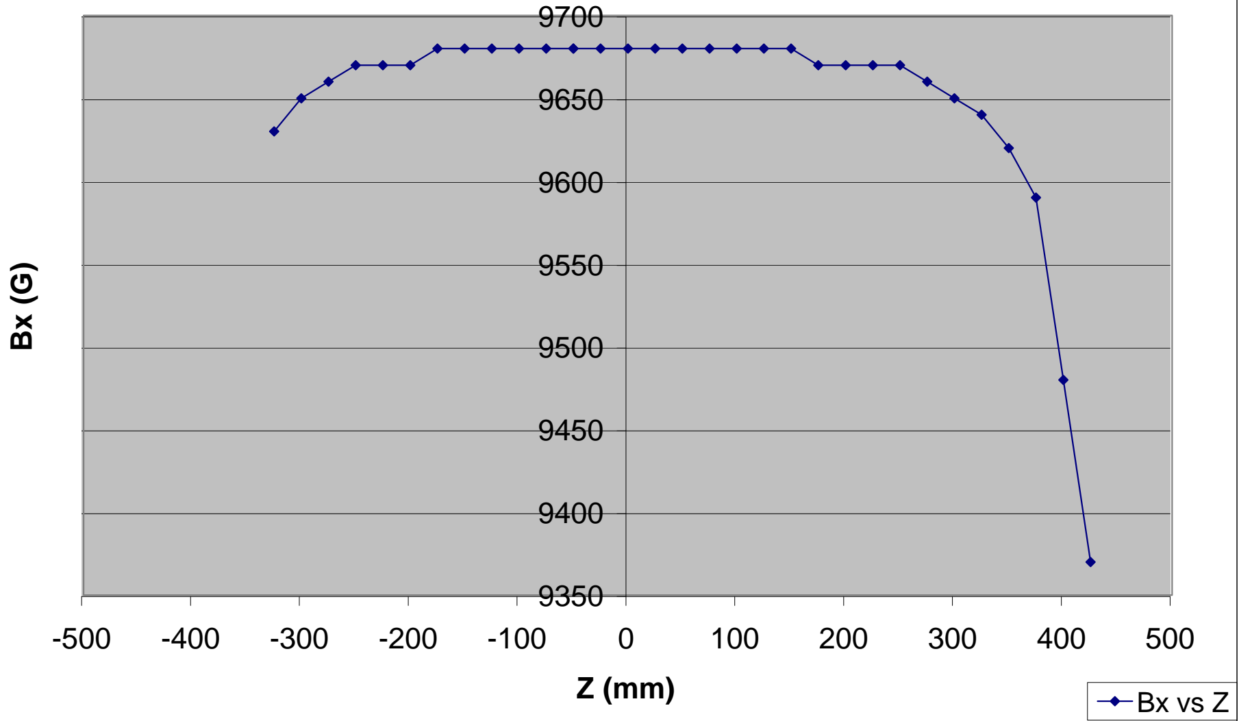
Bx vs Z at X=0, Y=0, I=500A
